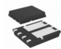
SI7940DP-T1-GE3 Vishay Siliconix MOSFET 2N-CH 12V 7.6A PPAK SO-8
