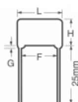
ECQ-P1H331JZ3 Panasonic Electronic Components CAP FILM 330PF 5% 50VDC RADIAL
