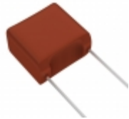
ECW-F2475HA Panasonic Electronic Components CAP FILM 4.7UF 3% 250VDC RADIAL
