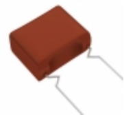
ECW-F2475JAQ Panasonic Electronic Components CAP FILM 4.7UF 5% 250VDC RADIAL
