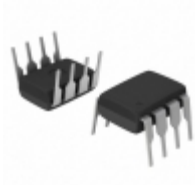
MCP4142-503E/P Microchip Technology IC DGTL SNGL 50K SPI 8DIP
