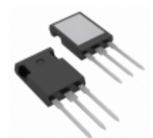
IXFR20N120P IXYS MOSFET N-CH 1200V 13A ISOPLUS247
