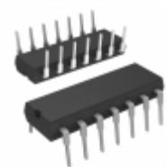
MCP4241-503E/P Microchip Technology IC DGTL POT DL 50K 2CH 14-DIP
