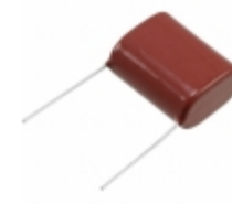
ECQ-E6225JFB Panasonic Electronic Components CAP FILM 2.2UF 5% 630VDC RADIAL
