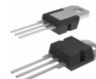
STP3LN80K5 STMicroelectronics MOSFET N-CHANNEL 800V 2A TO220
