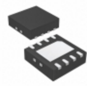
TC4452VMF713 Micrel / Microchip Technology IC MOSFET DVR 12A HS 8DFN
