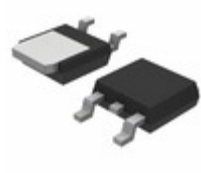
MBRD835LT4G ON Semiconductor DIODE SCHOTTKY 35V 8A DPAK
