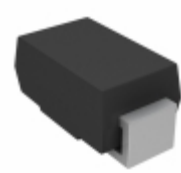
SMAJ48-E3/61 Vishay Semiconductor Diodes Division TVS DIODE 48VWM 85.5VC SMA
