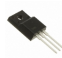
DPG20C300PN IXYS DIODE ARRAY GP 300V 10A TO220FP
