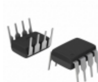
PS7141-2B-A CEL SSR OCMOS FET 150MA NC 8-DIP
