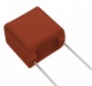
ECW-F2685JA Panasonic Electronic Components CAP FILM 6.8UF 5% 250VDC RADIAL
