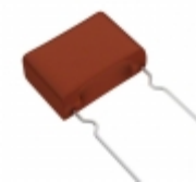
ECW-F2684RHA Panasonic Electronic Components CAP FILM 0.68UF 3% 250VDC RADIAL
