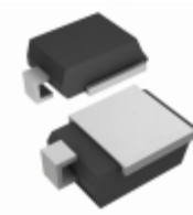
SM5S14A-E3/2D Vishay Semiconductor Diodes Division TVS DIODE 14VWM 23.2VC DO218AB
