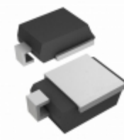
SM5S14AHE3/2D Vishay Semiconductor Diodes Division TVS DIODE 14VWM 23.2VC DO218AB
