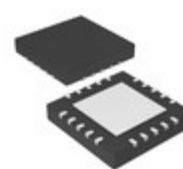
PIC24F08KA101-I/MQ Microchip Technology IC MCU 16BIT 8KB FLASH 20QFN
