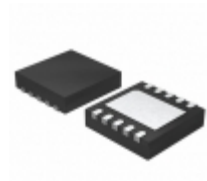
MCP4232-103E/MF Microchip Technology IC POT DGTL DUAL 10K RHEO 10DFN
