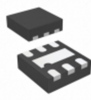
MIC5323-2.8YMT-TR Microchip Technology IC REG LDO 2.8V 0.3A 6TMLF
