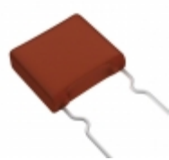
ECW-F2564JAB Panasonic Electronic Components CAP FILM 0.56UF 5% 250VDC RADIAL
