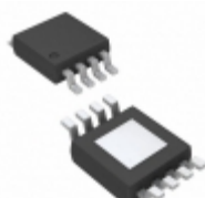
MIC47100-12YMME-TR Microchip Technology IC REG LDO 1.2V 1A 8MSOP
