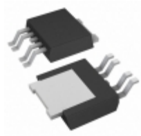
BA05CC0WFP-E2 Rohm Semiconductor IC REG LDO 5V 1A TO252-5
