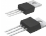
MC7912CT-BP Micro Commercial Co IC REG LDO -12V 1.5A TO220
