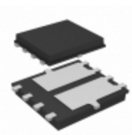
SI7220DN-T1-E3 Electro-Films (EFI) / Vishay MOSFET 2N-CH 60V 3.4A 1212-8
