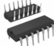
TS934AIN STMicroelectronics IC OPAMP GP 100KHZ RRO 14DIP
