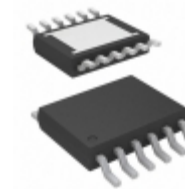
LT3015EMSE-2.5#TRPBF ADI (Analog Devices, Inc.) IC REG LINEAR -2.5V 1.5A 12MSOP
