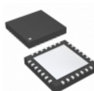
PIC24FV08KM202-E/ML Microchip Technology IC MCU 16BIT 8KB FLASH 28QFN
