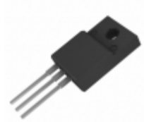
FQPF50N06L Fairchild/ON Semiconductor MOSFET N-CH 60V 32.6A TO-220F
