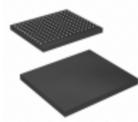
CY7C1414KV18-250BZCT Cypress Semiconductor Corp IC SRAM 36MBIT 250MHZ 165FBGA
