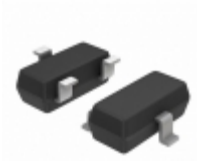
BCX17LT3G ON Semiconductor TRANS PNP 45V 0.5A SOT-23
