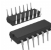
DM74ALS37AN Fairchild/ON Semiconductor IC GATE NAND 4CH 2-INP 14-DIP
