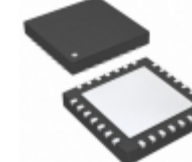
PIC16F72T-1/ML Microchip Technology IC MCU 8BIT 3.5KB FLASH 28QFN
