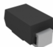
SML4753-E3/61 Electro-Films (EFI) / Vishay DIODE ZENER 36V 1W DO214AC
