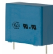
B32914A3105K189 EPCOS (TDK) CAP FILM 1UF 10% 760VDC RADIAL
