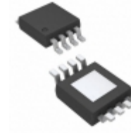
AP2145MPG-13 Diodes Incorporated IC SINGLE USB SWITCH 800MA 8MSOP
