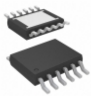
LT3065HMSE-1.5#PBF Linear Technology IC REG LDO 1.5V 0.5A 12MSOP
