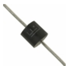
5KP15CA Littelfuse Inc. TVS DIODE 15VWM 24.4VC P600
