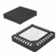
PIC16F1778-I/MX Microchip Technology IC MCU 8BIT 28KB FLASH 28UQFN
