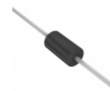
1.5KE33CA-E3/73 Vishay Semiconductor Diodes Division TVS DIODE 28.2VWM 45.7VC 1.5KE
