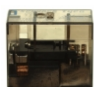
XT424024 Agastat Relays / TE Connectivity RELAY GEN PURPOSE DPDT 8A 24V
