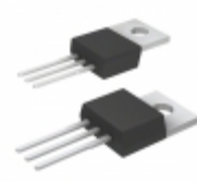
MCP1827S-1802E/AB Microchip Technology IC REG LDO 1.8V 1.5A TO220-3
