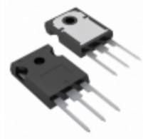
STGW40NC60KD STMicroelectronics IGBT 600V 70A 250W TO247
