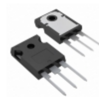
STGW40NC60WD STMicroelectronics IGBT 600V 70A 250W TO247
