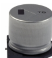
EEV-TG1K471M Panasonic Electronic Components CAP ALUM 470UF 20% 80V SMD
