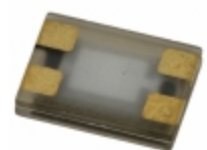
FQ7050B-6.000 Fox Electronics CRYSTAL 6.0000MHZ 20PF SMD
