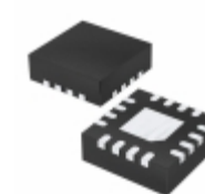
MCP4231T-103E/ML Microchip Technology IC POT DGTL DUAL 10K SPI 16QFN
