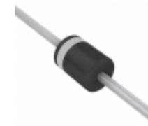
GI826-E3/54 Vishay Semiconductor Diodes Division DIODE GEN PURP 600V 5A P600
