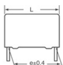
B32923C3564K000 EPCOS CAP FILM 0.56UF 10% 305VAC RAD
