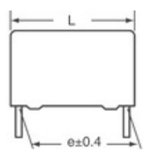
B32923C3564K EPCOS (TDK) CAP FILM 0.56UF 10% 305VAC RAD
