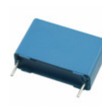
B32923C3474M289 EPCOS (TDK) CAP FILM 0.47UF 20% 305VAC RAD
