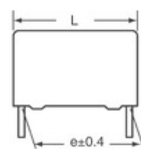
B32923C3564M189 EPCOS (TDK) CAP FILM 0.56UF 20% 305VAC RAD
