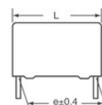
B32923C3564K289 EPCOS (TDK) CAP FILM 0.56UF 10% 305VAC RAD
