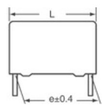
B32923C3564M289 EPCOS (TDK) CAP FILM 0.56UF 20% 305VAC RAD
