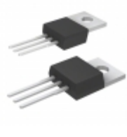
MCP1827S-2502E/AB Microchip Technology IC REG LDO 2.5V 1.5A TO220-3
