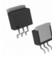
MCP1827S-2502E/EB Microchip Technology IC REG LDO 2.5V 1.5A 3DDPAK
