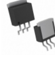
MCP1827S-3002E/EB Microchip Technology IC REG LDO 3V 1.5A 3DDPAK
