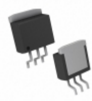
MCP1827S-1802E/EB Microchip Technology IC REG LDO 1.8V 1.5A 3DDPAK
