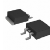
FFB10UP20STM Fairchild/ON Semiconductor DIODE GEN PURP 200V 10A D2PAK
