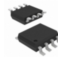
IRF7351TRPBF Infineon Technologies MOSFET 2N-CH 60V 8A 8-SOIC
