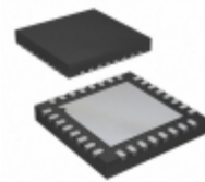
ADM3315EACPZ Analog Devices Inc. IC TXRX RS-232 3:3 2.7V 32LFCSP
